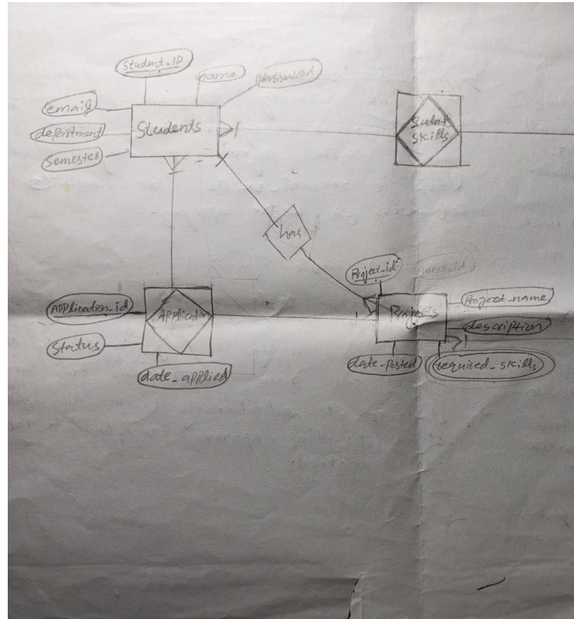
Fig. 1. Entity Relationship Diagram (ERD) of Campus Collaboration Finder
