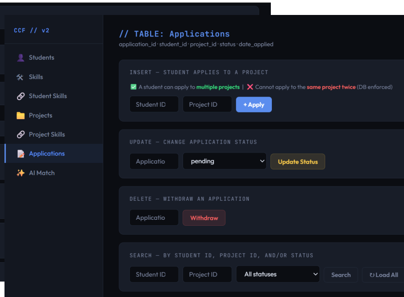
Fig. 4. Applications Management Interface
