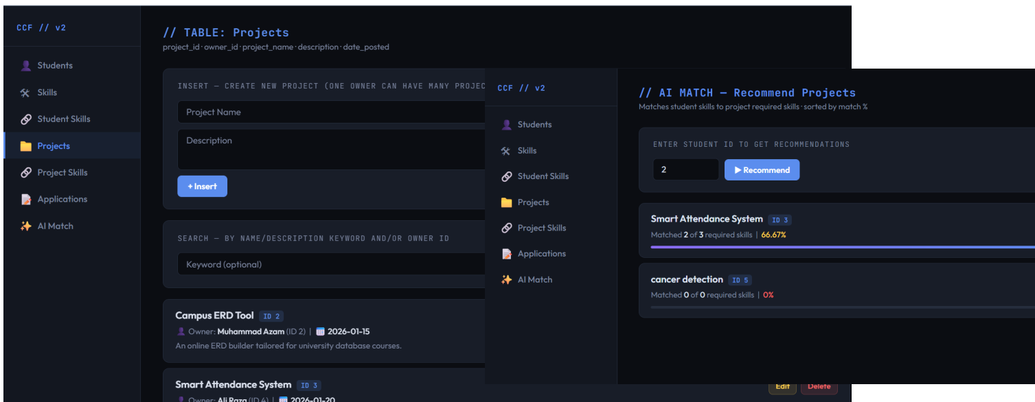
Fig. 5. AI-Powered Project Recommendation Interface
