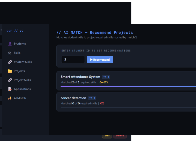
Fig. 5. AI-Powered Project Recommendation Interface
